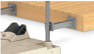
Telescoping Port to Fixed Dock Kit Adjusts from 41 to 61 cm. 301434 - Fits 2" Pipe 301435 - Fits 4" Pipe
