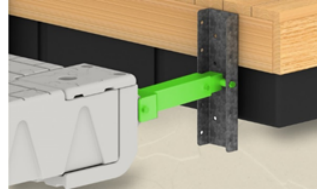
Alu. Extension Arm Kit 301436 - Adjusts from 41 to 61 cm (2qty) Use for SLX series part no. 301308
